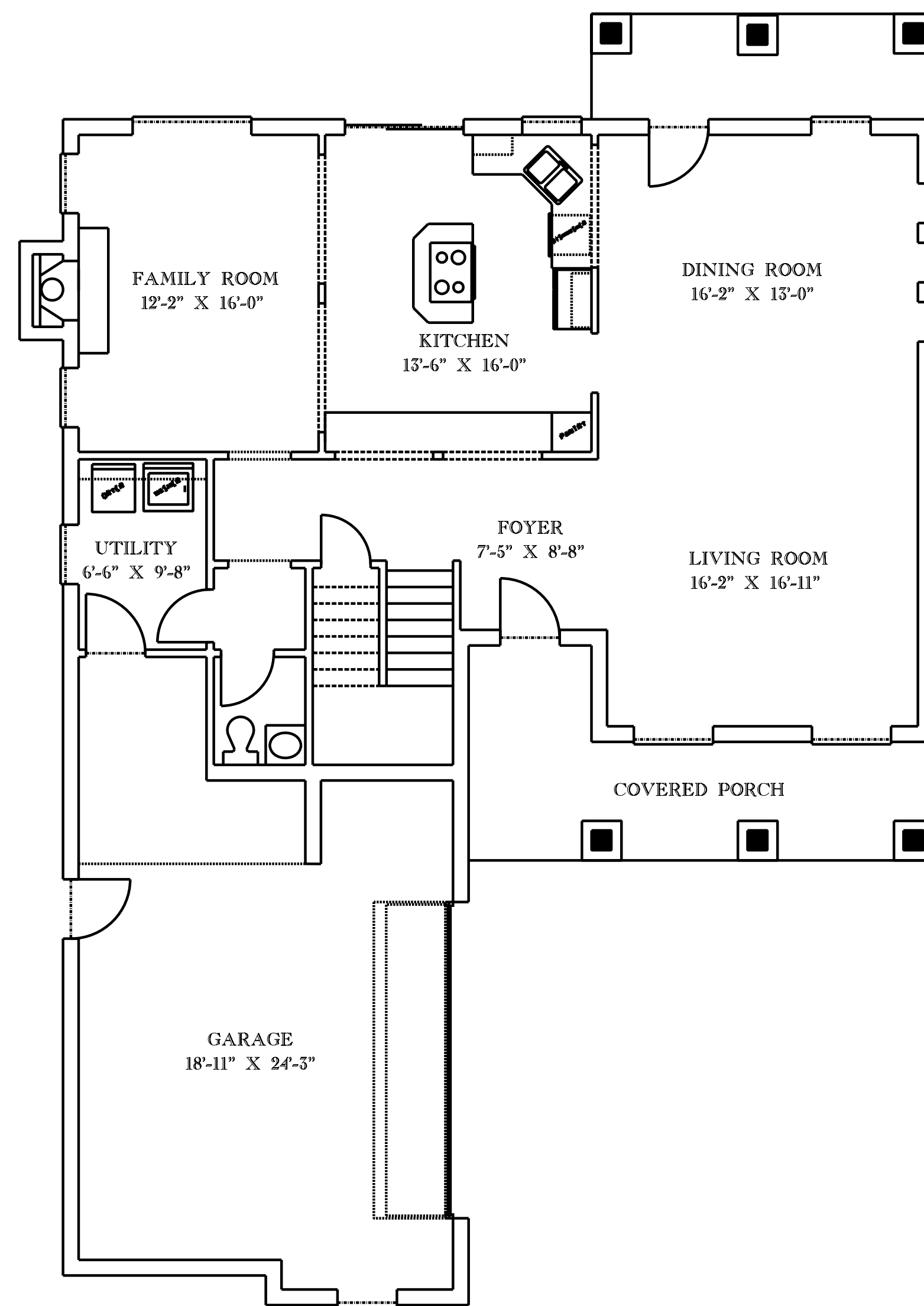
FIRST FLOOR
